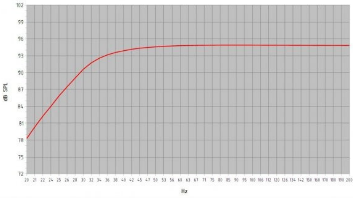
Frequency Response (2 Vrms/1 m)
